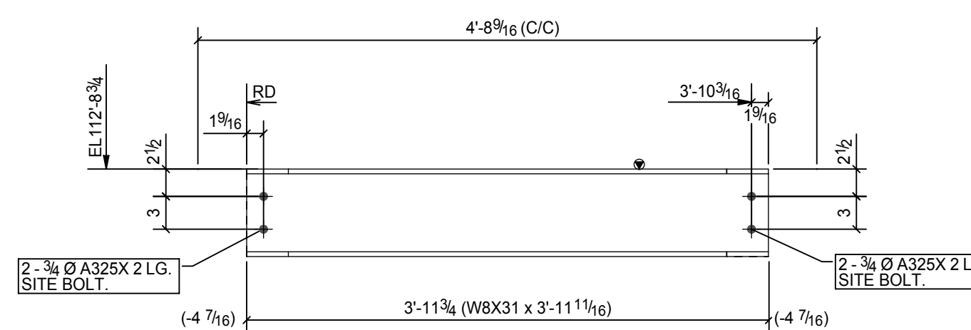
ONE - BEAM - 35B9
