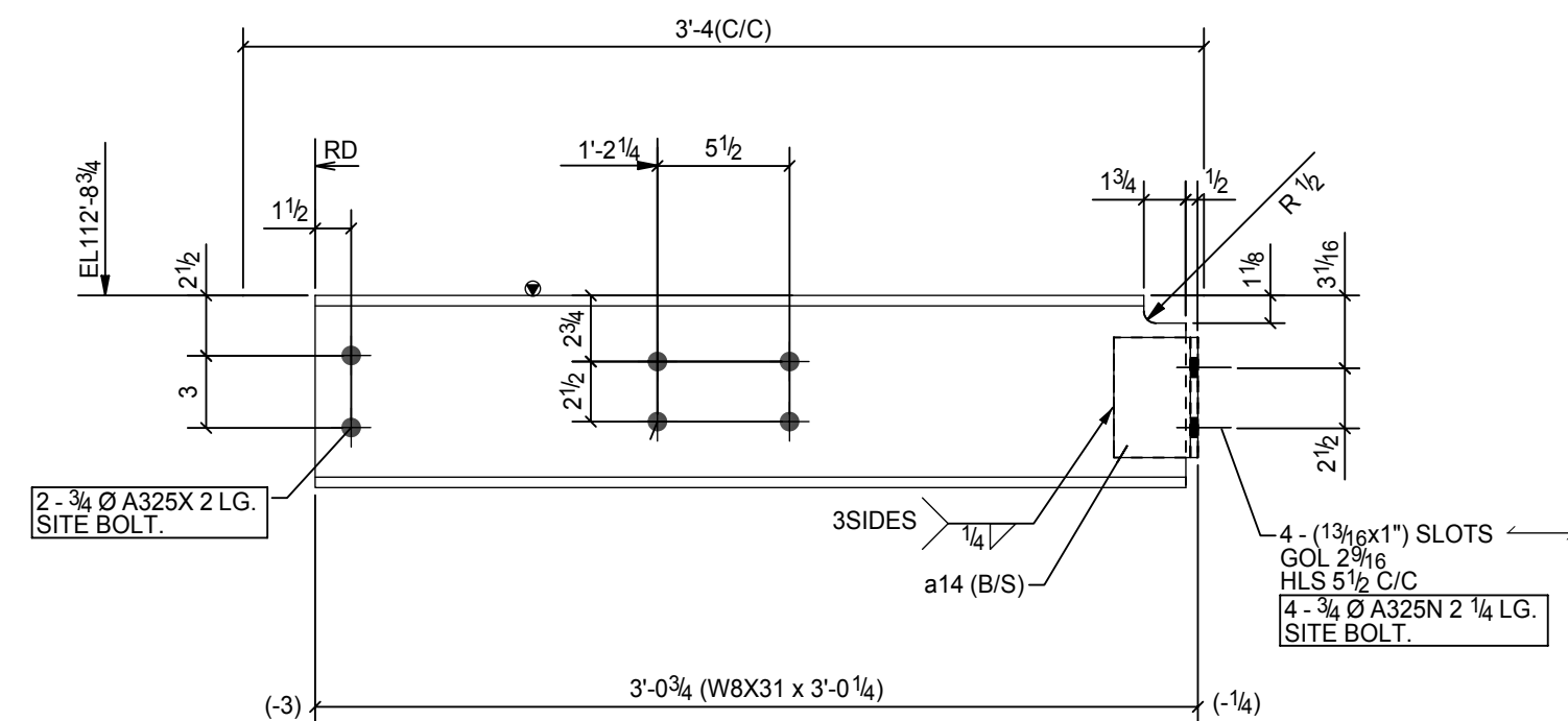
ONE - BEAM - 35B2 (ANGLE 3 1/2 LEG WELDED WITH BEAM)
