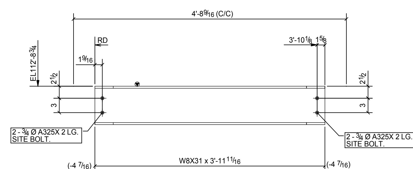
ONE - BEAM - 35B4
