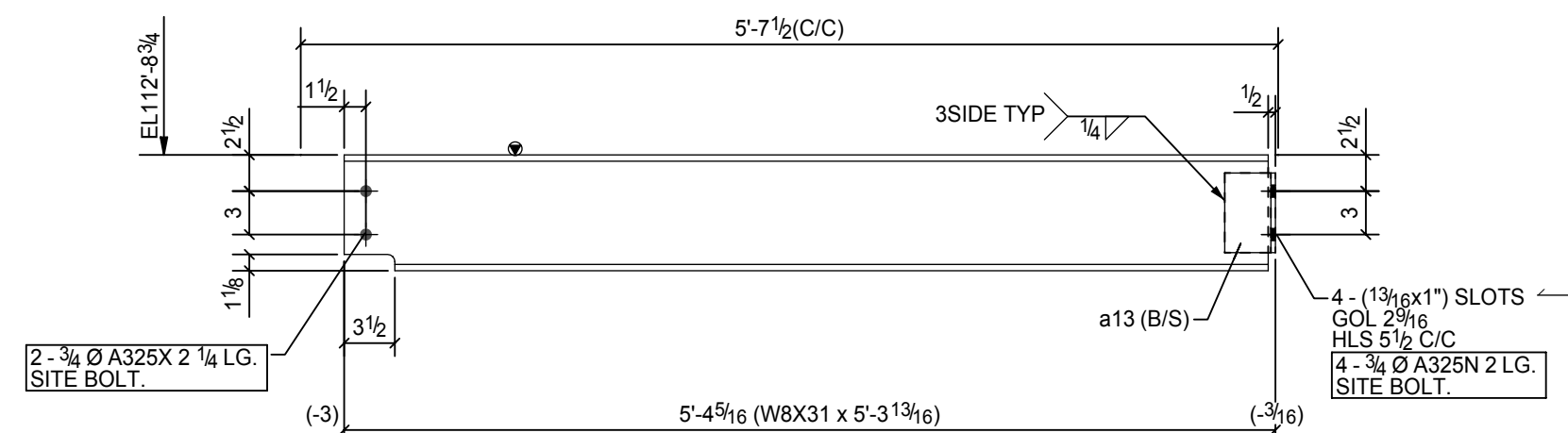
2 - BEAMS - 35B7 (ANGLE 3 1/2 LEG WELDED WITH BEAM)
