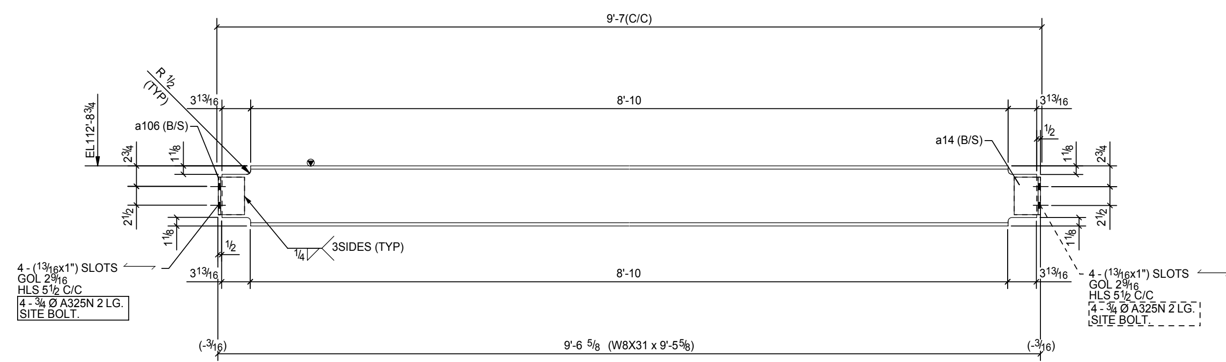
ONE - BEAM - 35B1 (ANGLE 3 1/2 LEG WELDED WITH BEAM)
